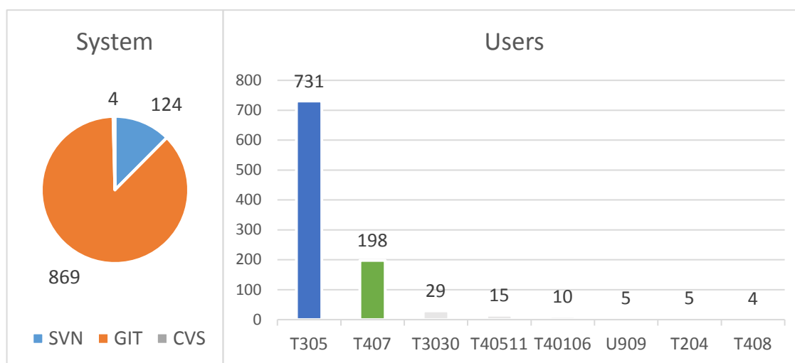
Fig.1 Statistic of different system usage based on interviews and a preliminary report [3]
