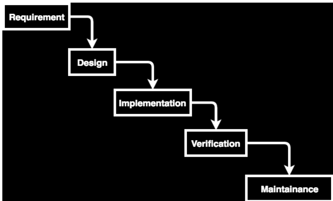
Figure 9: Waterfall process
