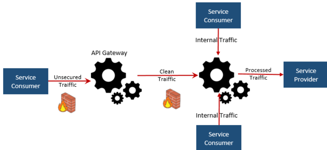
Fig 19 – API Gateway
