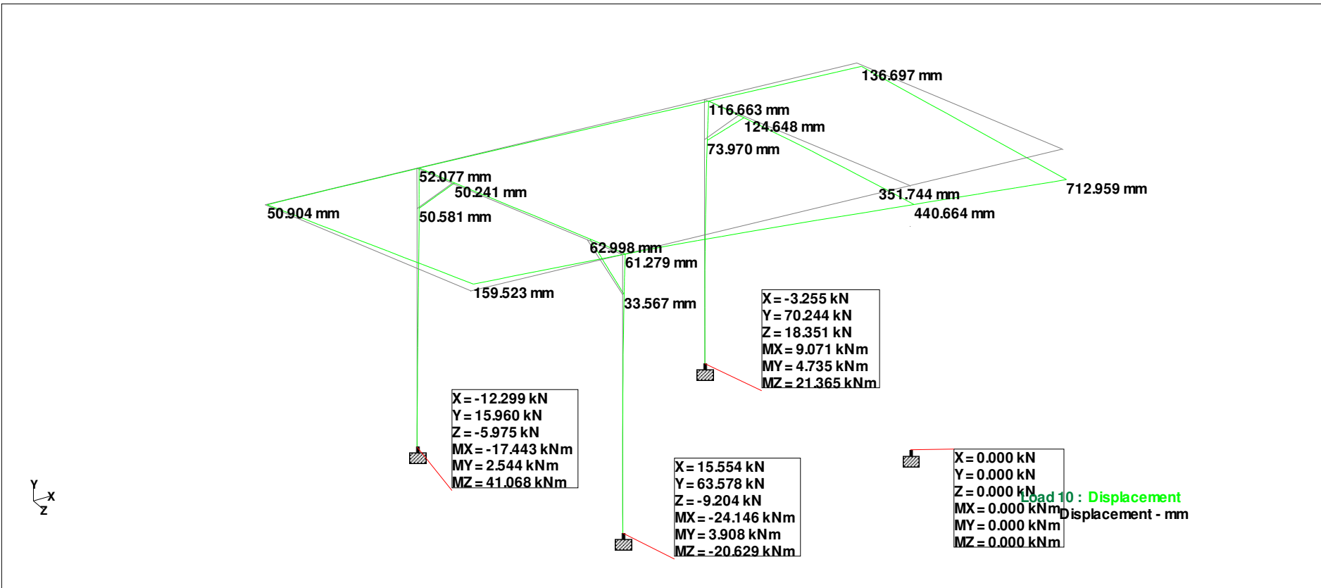
Whole Structure Displacements 1000mm:1m 10 ACC PILARI POIS 1+ Reactions
