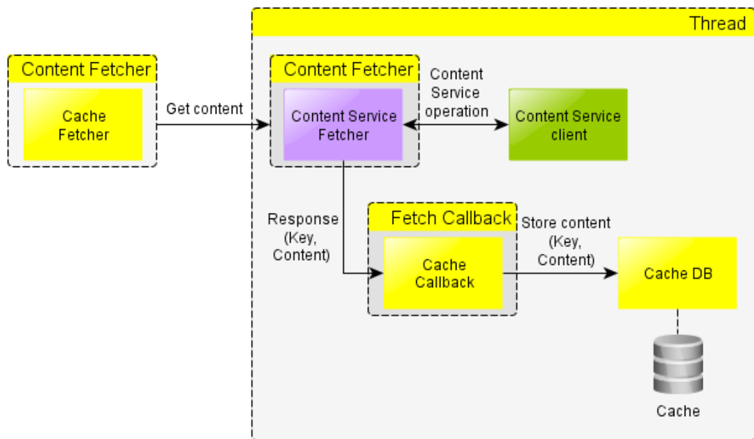
Figure 10. Asynchronous “Fetch Callback”
